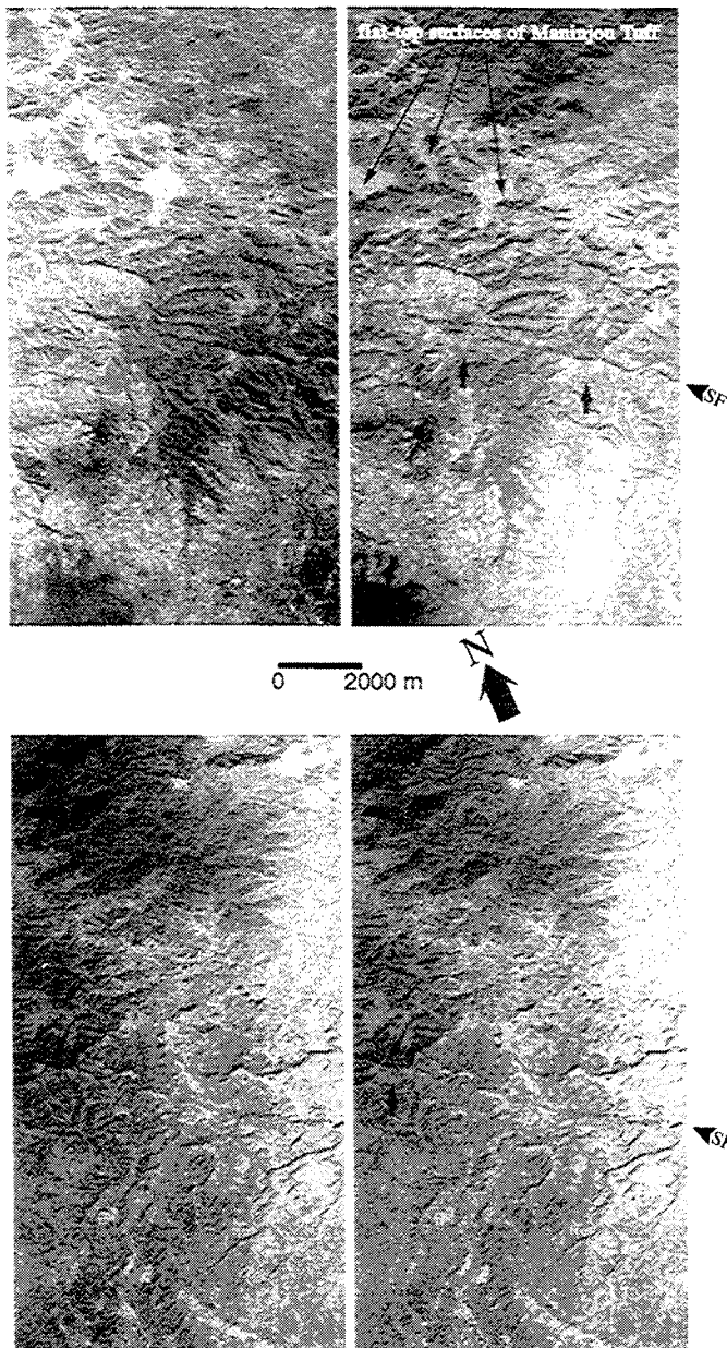
Figure 3. An example of the approximately 1:100,000-scale aerial photographs we used to compile most of our map of the Sumatran fault. These two sets of stereopairs show channel offsets of ~720 m. The channels cut a late Pleistocene pyroclastic flow deposit at about 0.3^{\circ}\text{S} . The flat upland surfaces are the unincised top of the flow. These offsets yield a average slip rate of ~11 mm/yr.
