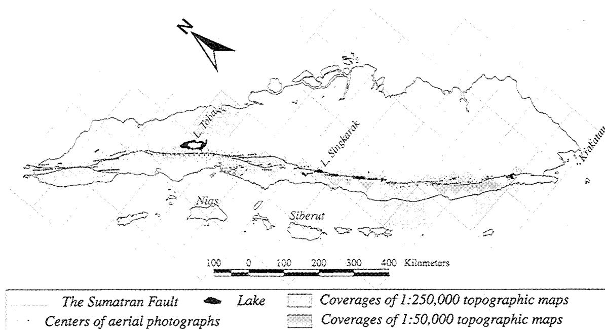
Figure 2. Data upon which our map compilation is based. Most of our mapping is based on inspection of 1:50,000-scale topographic maps produced by BAKOSURTANAL & JANTOP, the national mapping agencies for Indonesia, and 1:100,000-scale aerial photographs. Other data sources include smaller-scale geologic and topographic maps.
