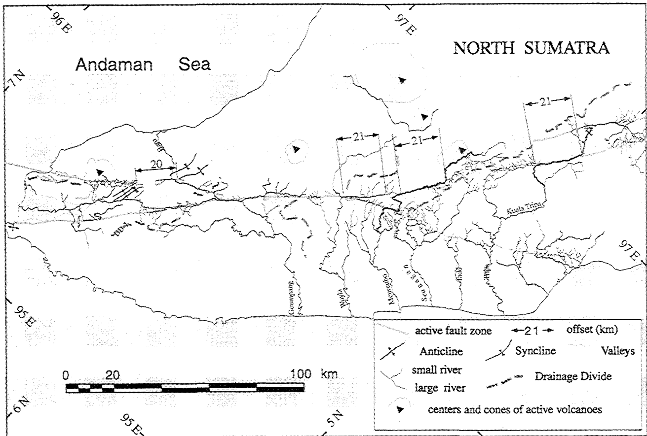
Figure 7. Two of the most compelling large geomorphic offsets along the Sumatran fault, the 21-km dextral offsets of the Tripa and Meureubo Rivers in north Sumatra. The headwaters of the nearby Woyla River and folded Quaternary sediments near 6°N also appear to be offset by this amount. These offsets appear to represent the total dextral offset since initial uplift of this part of the Barisan Mountains several million years ago.
