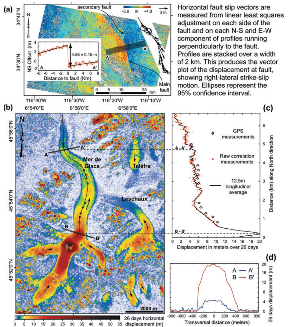
Fig. 1. (a) North/south component (northward positive) of the coseismic displacement field due to the 1999 Hector Mine earthquake, California. The pre-earthquake image (10-meter SPOT 4 acquisition from 17 August 1998) and the post-earthquake image (15-meter ASTER acquisition from 10 May 2000) were orthorectified and coregistered on a 10-meter-resolution grid, and offsets were measured from subpixel correlation between sliding windows. No measurement is assigned to white points where the correlation is too weak. The main fault rupture is a linear discontinuity in the data. The standard deviation on individual measurements is around 1.3 meters. (b) Amplitude of the horizontal displacement over the Mer de Glace area from 23 August 2003 to 18 September 2003, obtained from two panchromatic 2.5-meter-resolution SPOT 5 images. Arrows indicate the flow direction. Displacements below the images' resolution appear in blue. Displacements as high as 55 meters (about 800 meters per year) are recorded over this 26-day period. (c) Displacements along a central flow line of the Mer de Glace measured from SPOT 5 images and from campaign GPS. The time period covered by the GPS (12 August 2003 to 3 September 2003) starts slightly earlier in the summer and includes the August 2003 European heat wave, which explains the faster velocities observed over this period [ Berthier et al., 2005 ]. (d) Displacement along transverse profiles AA' and BB'.
